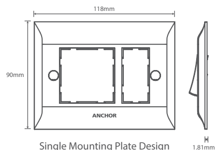
Single Mounting Plate Design
